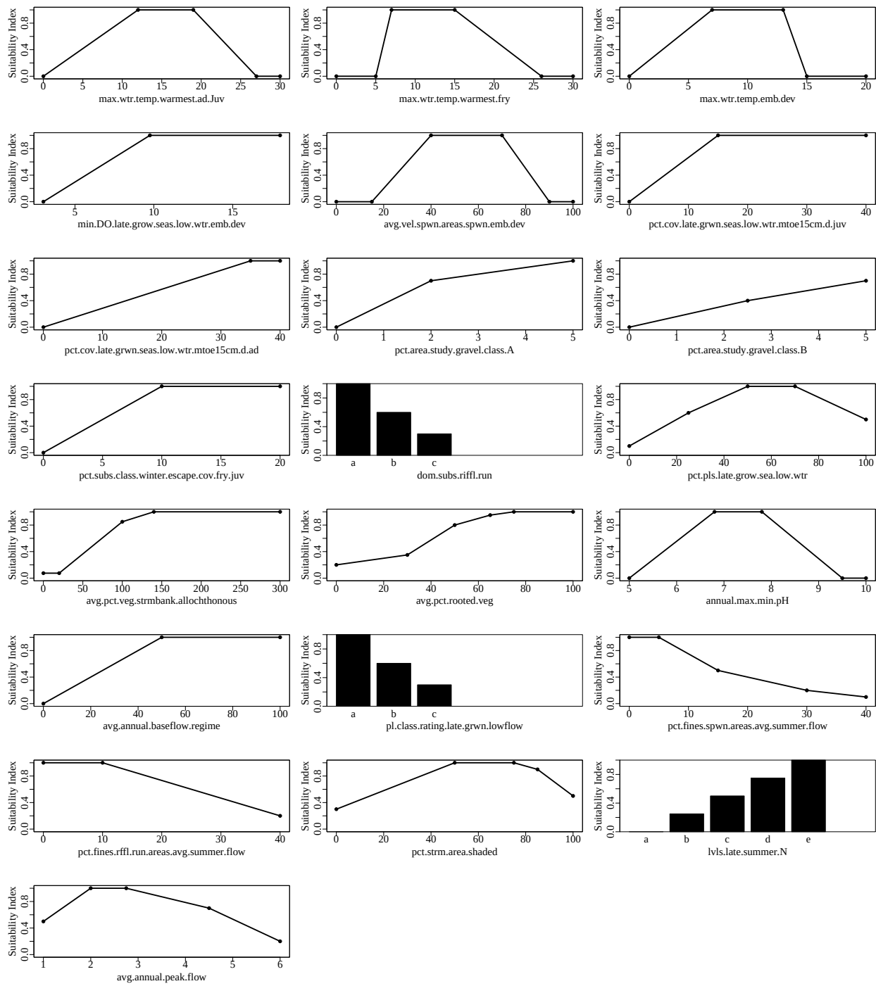
Figure 1. Suitability index graphs for variables included in the browntroutLimitLtoe10C model in ecoest.
