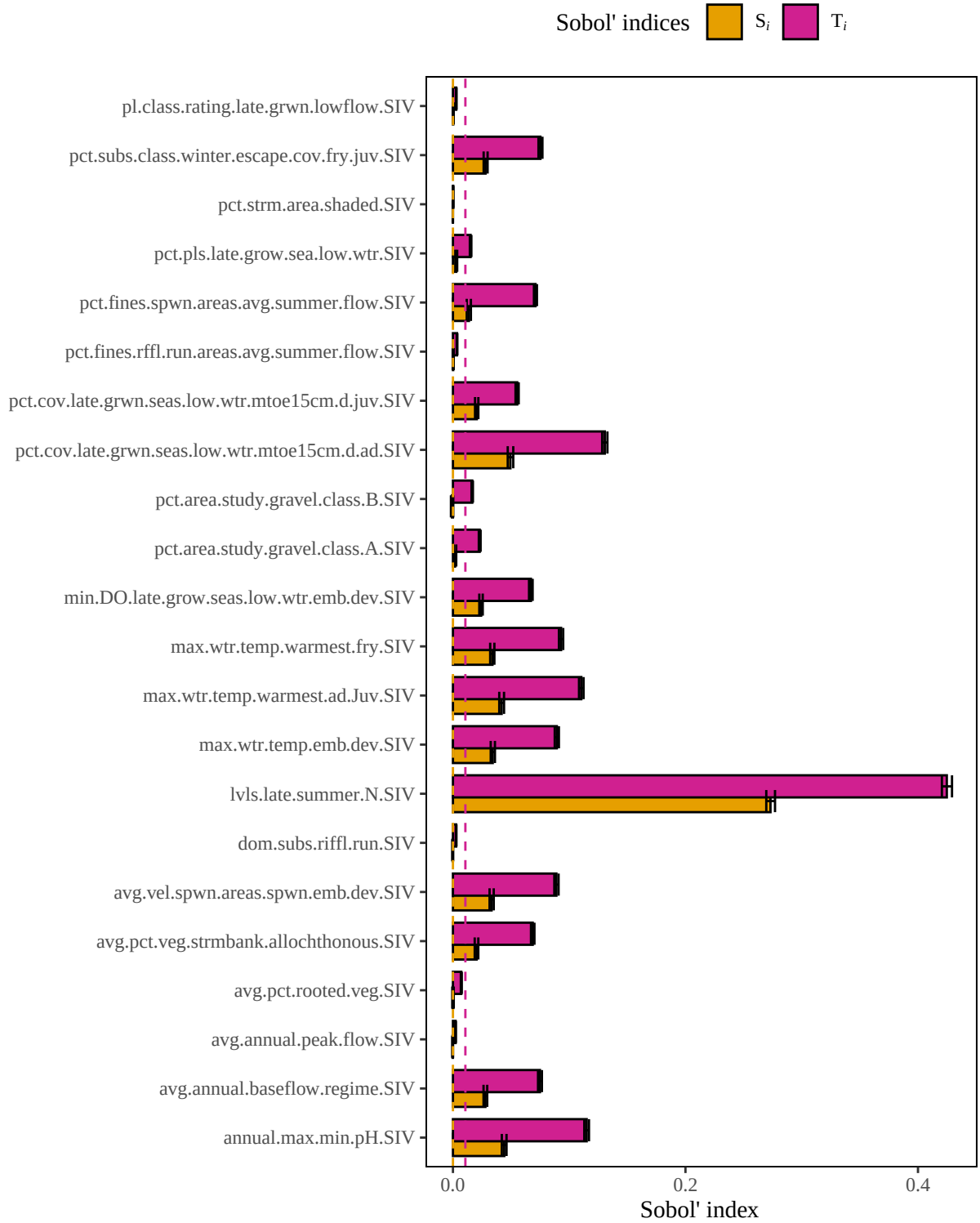
Figure 3. Results of a sensitivity analysis for the browntROUTLimitLtoe10C model based on the original limiting factor model outlined in Raleigh et al. (1986). Dashed lines represent baseline numerical approximation error for S_i and T_i ( i.e. , dummy variables).
