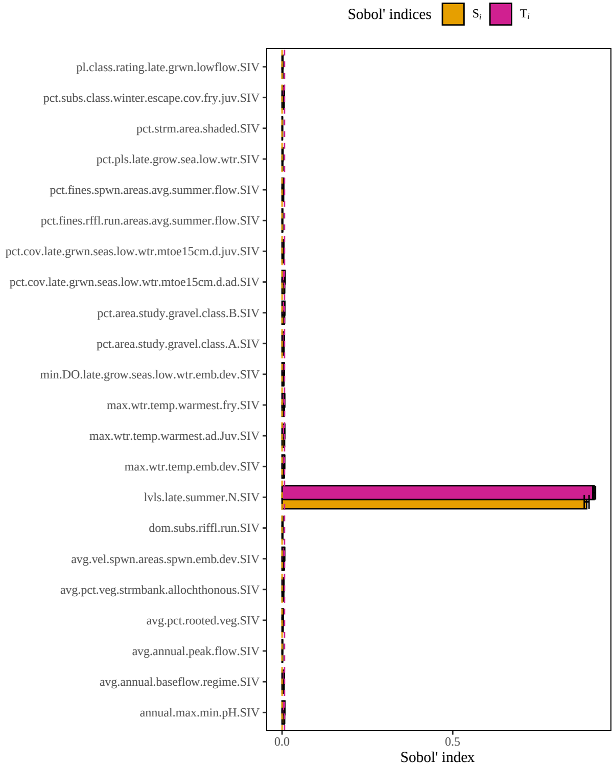
Figure 5. Results of a sensitivity analysis for the browntROUTLimitLtoe10C model based on a geometric mean structure. Dashed lines represent baseline numerical approximation error for S_i and T_i ( i.e. , dummy variables).
